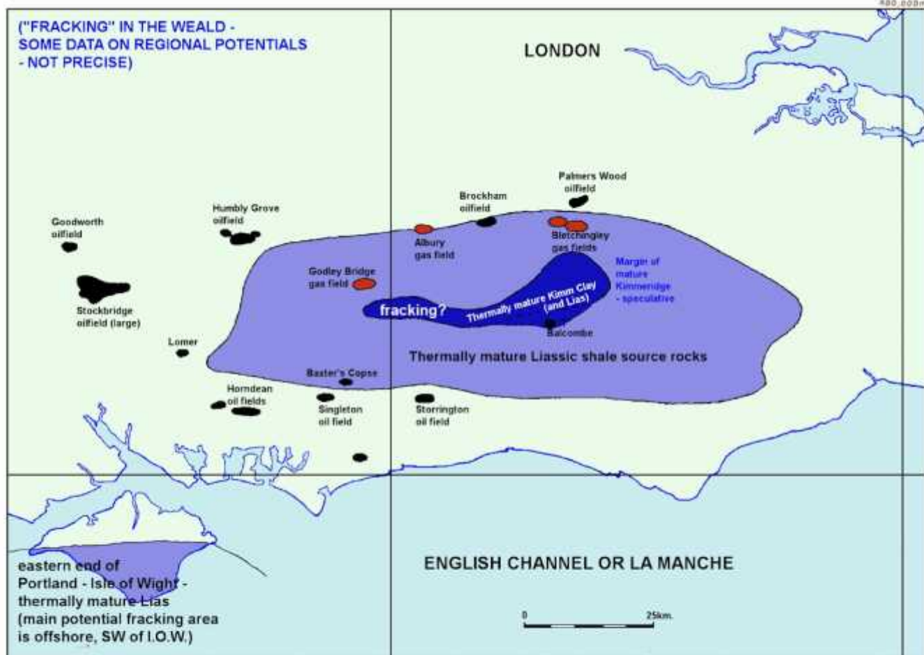
MATURE, JURASSIC SOURCE ROCKS AREAS FOR THE WEALD BASIN, AS POSTULATED BY BUTLER AND PULLAN (1990). This has been given for the end-Cretaceous, but since there is no Tertiary over the central area it is reasonably applicable for the present. The mature Kimmeridge Clay are speculative, but the general area delineated is likely to be correct. Balcombe, the fracking locality, may be Kimmeridge Clay (but it seems likely). The dark blue area (Kimmeridge mature) may be most favourable for fracking because there is no Tertiary over it. However, areas beyond, with only mature Liassic shales could be subject to fracking in the future. (The map has been redrawn with reference to Butler and Pullan, 1990, Tertiary Structures and Hydrocarbon Entrapment in the Weald Basin of Southern England, an interesting paper in Journal of Petroleum Geology , 1990, 12, 1-12, and Ian West, 2013, Oil & Gas Geology of the Weald Basin , 2013, 1-12).
